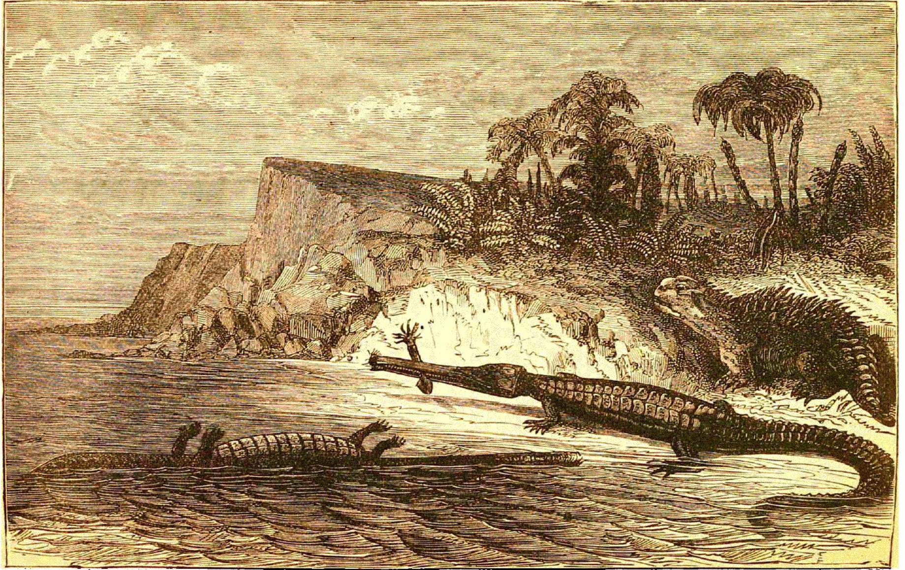
XVIII.—Ideal landscape of the Middle Oolitic Period.
