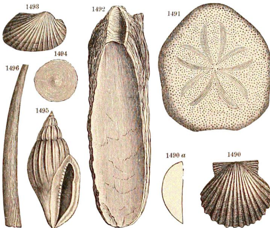
EOCENE. — Vicksburg group . — Fig. 1490, Pecten Poulsoni ; a , section of same; 1491, Mortonia Rogersi ; 1492, Ostrea Georgiana ( \times \frac{1}{2} ), Vicksburg (?); 1493, Arca Mississippensis ; 1494, Orbitoides Mantelli ; 1495, Lyria costata ; 1496, Dentalium Mississippense . Figs. 1490-1492, 1494, Meek; 1493, 1495, 1496, Conrad.
