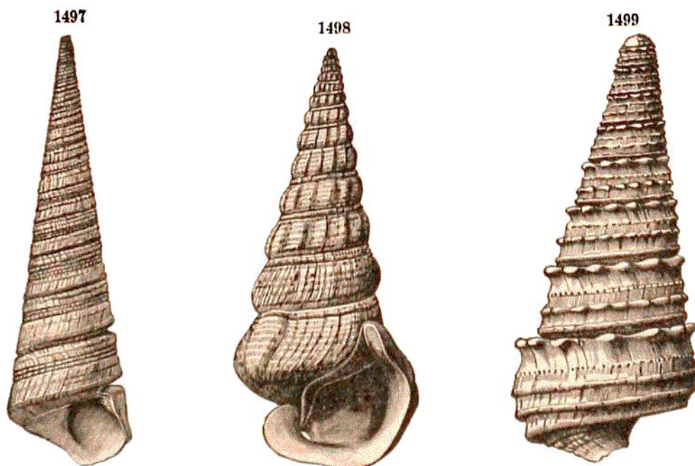
MIOCENE. — Chattahoochee group . — Fig. 1497, Turritella Tampae ( \times \frac{1}{2} ); 1498, Pyrazisinus campanulatus ; 1499, Cerithium Hillsboroense . From Dall.
