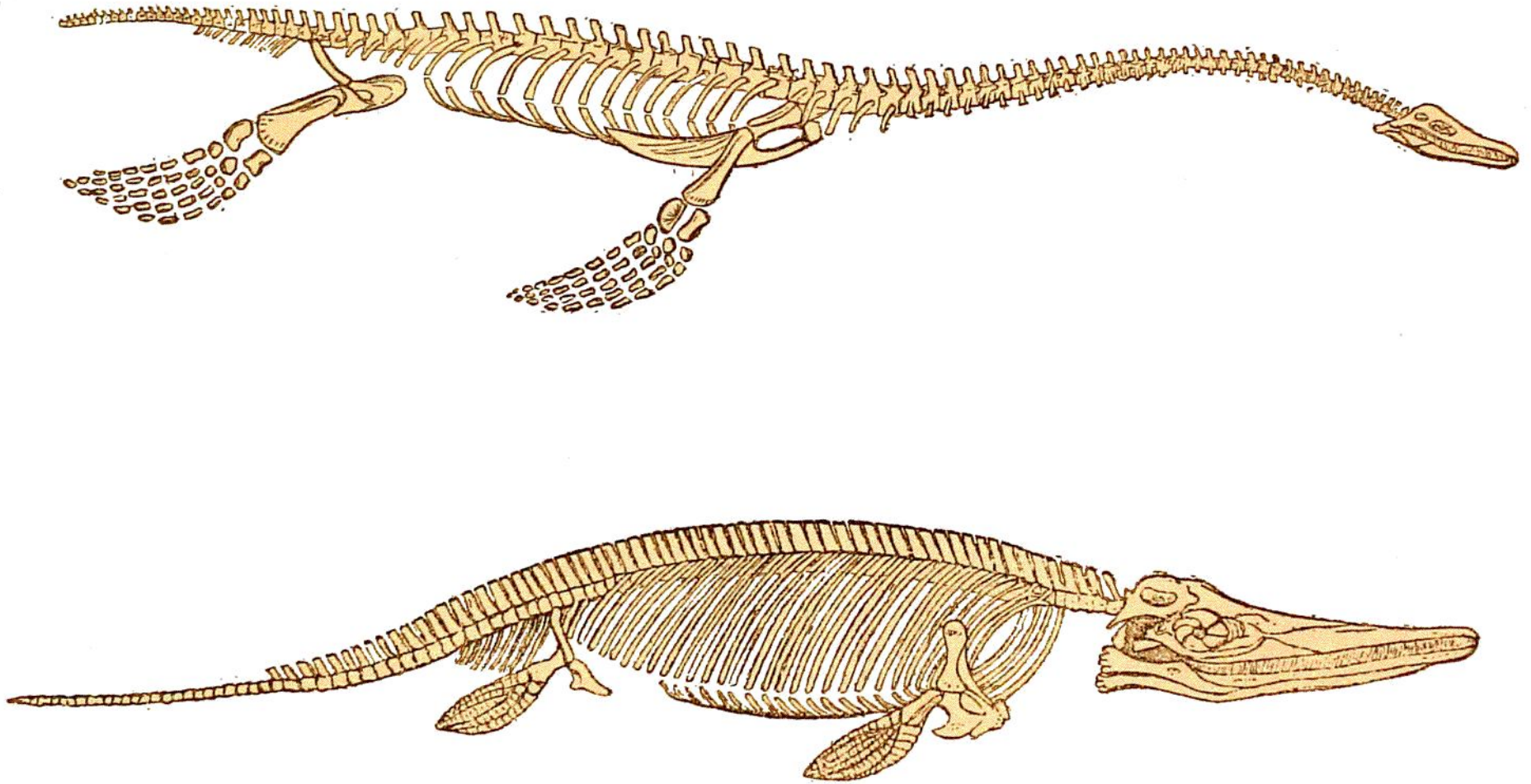
Fig. 396.—Jurassic Enaliosaurs or Sea-lizards. a , Ichthyosaurus communis , Conyb. (restored by Conybeare and Cuvier); b , Plesiosaurus dolichodeirus , Conyb. (restored by Conybeare).
